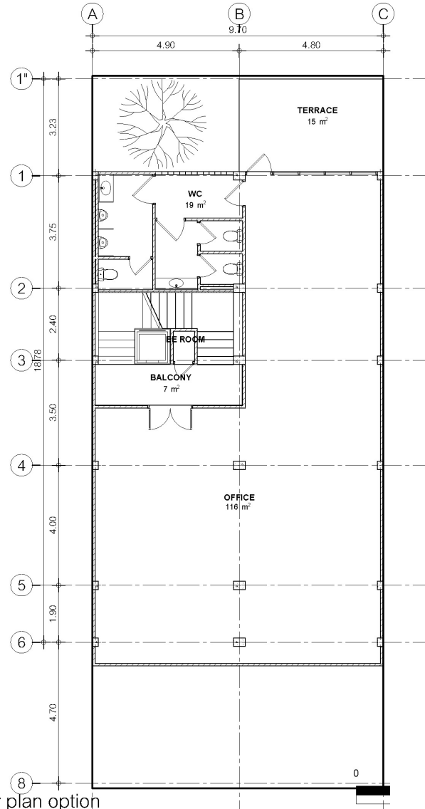
2nd Floor plan option
