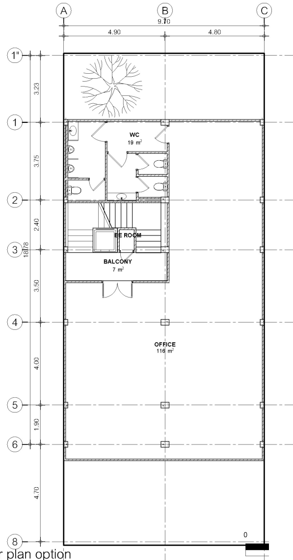
4th Floor plan option
